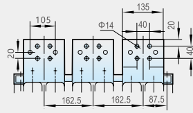
DW17D-2900(In = 2900A)
