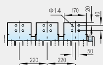
DW17D-3900(In=3200A)
