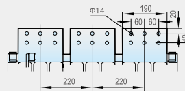
DW17D-3900(In=3900A)
