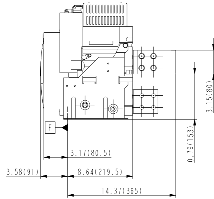
2500A_Type C_Veritical_Reverse
