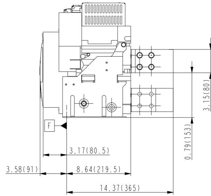
2500A_Type D_Vertical_Reverse
