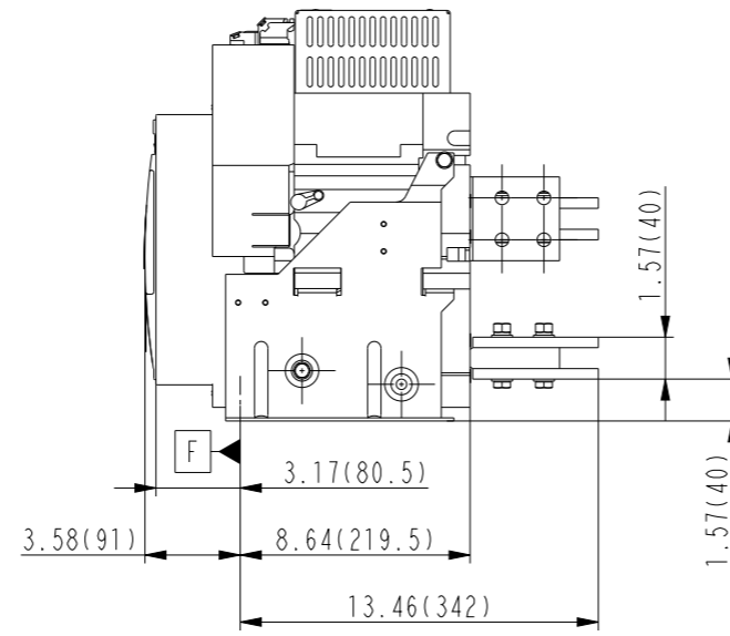
800_2000A_Type D_Vertical
