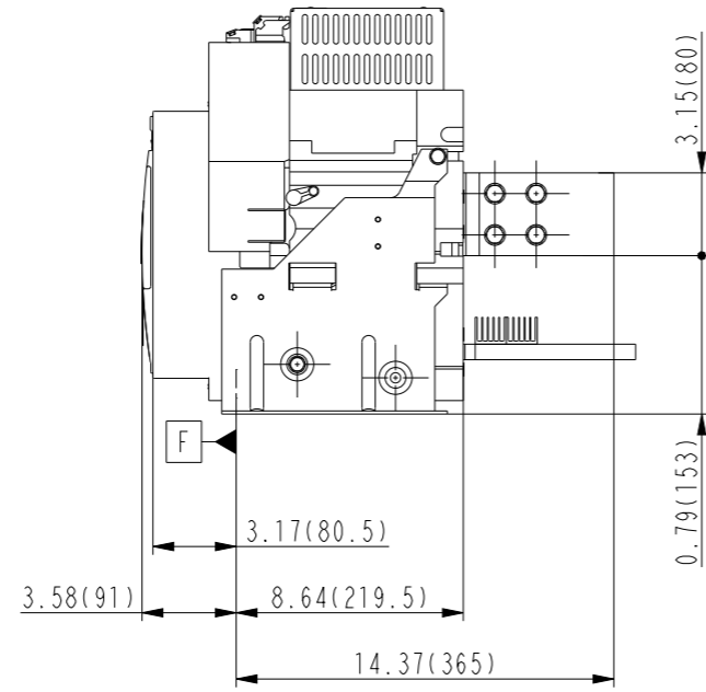
2500A_Type C_Horizontal_Reverse
