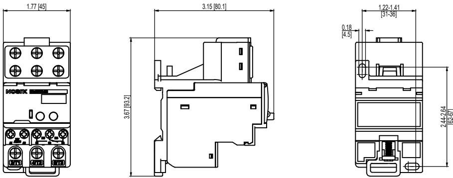
Ex9RE40+AD57 Unit: in [mm]
