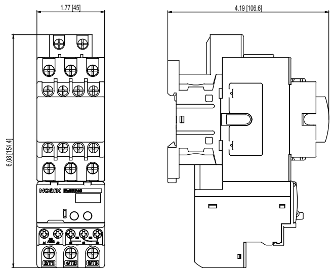
Ex9RE40+Ex9C25 - 38 Unit: in [mm]
