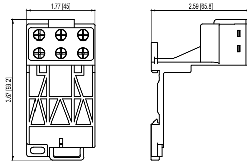
AD57 Unit: in [mm]
